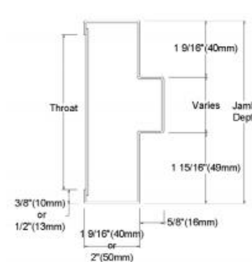
Single Rabbet
