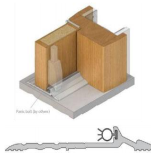
Threshold Plate Seal-RP117Si
