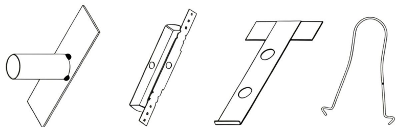
Wire Anchor T Anchor Universal Anchor Tube Anchor
