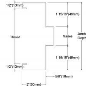
Double Rabbet
