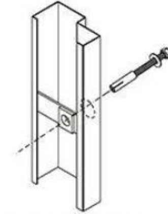
Expansion-Shell Anchor (Standard)
